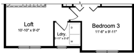
Opt. Upper Floor Plan ~ w/Loft 973 sq. ft.
