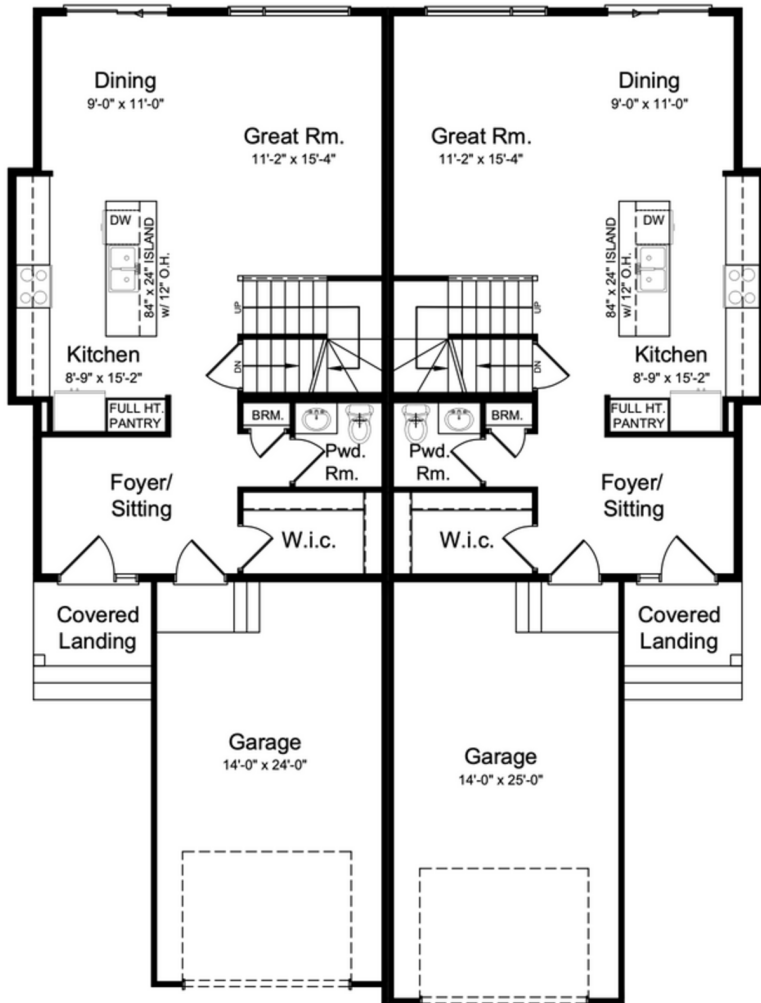
Main Floor Plan ~ 735 sq. ft. Upper Floor Plan ~ 770sq. ft. Total Area ~ 1505 sq. ft. ea. unit
