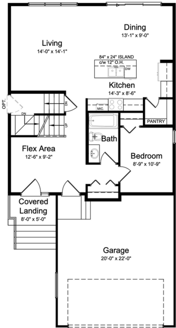
Main Floor Plan ~ 902 sq. ft. Upper Floor Plan ~ 896 sq. ft. Total Area ~ 1798 sq. ft.
