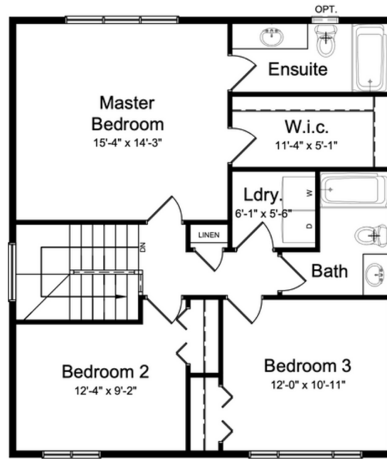
Upper Floor Plan ~ 896 sq. ft.
