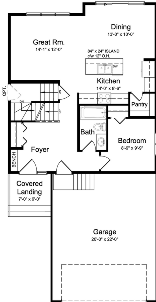
Main Floor Plan ~ 840 sq. ft.
