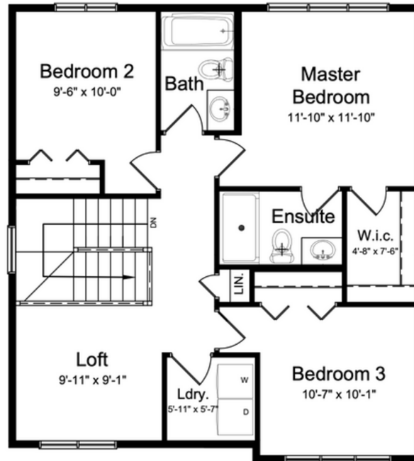
Upper Floor Plan ~ 851 sq. ft.
