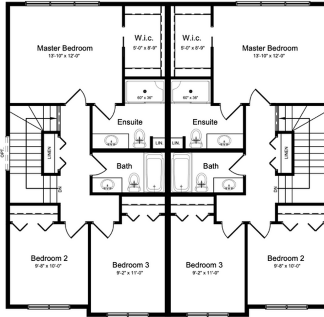
Upper Floor Plan ~ 770 sq. ft. ea. unit
