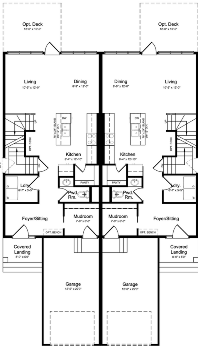
Main Floor Plan ~ 760 sq. ft. Upper Floor Plan ~ 770 sq. ft. Total Area ~ 1530 sq. ft.
