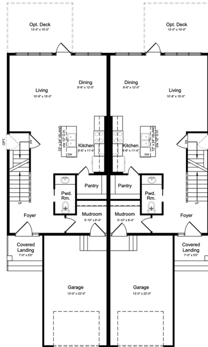
Main Floor Plan ~ 720 sq. ft. Upper Floor Plan ~ 744 sq. ft. Total Area ~ 1464 sq. ft.
